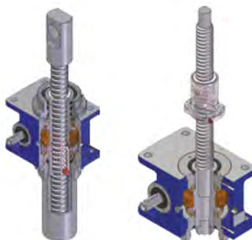
Ball screw jacks
